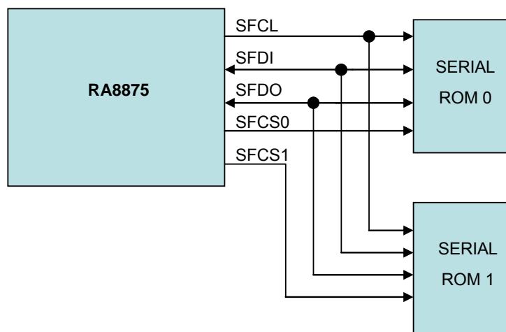
Figure 6-38 : RA8875 Serial Flash/ROM System
