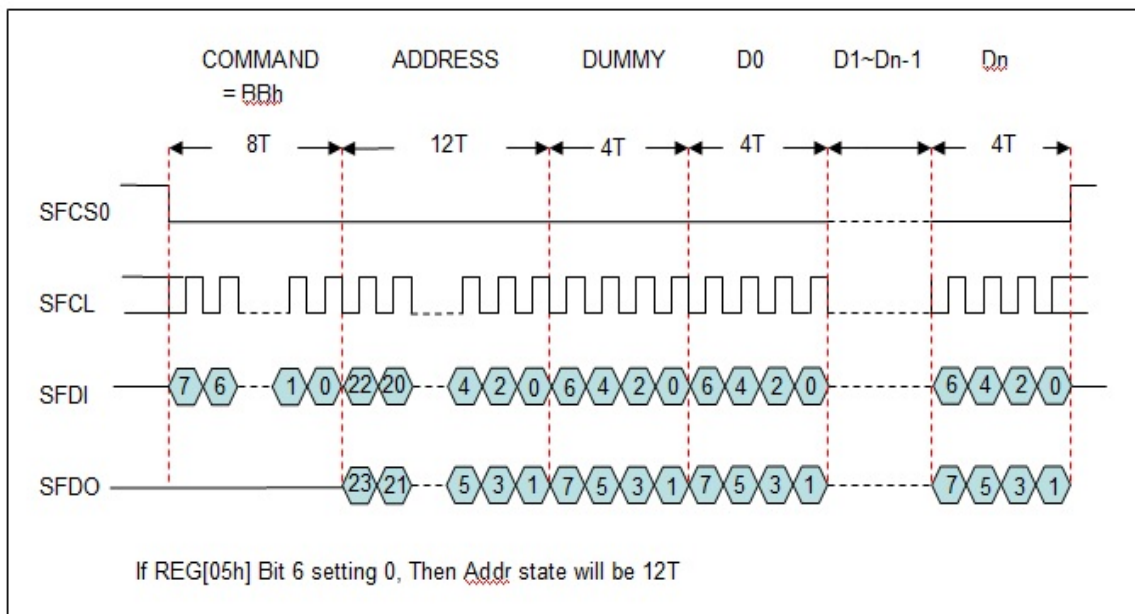
Figure 6-43 : Dual – 1 Read
