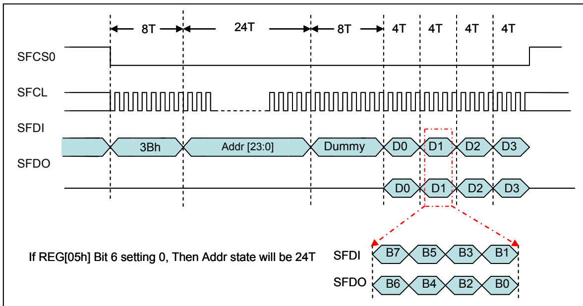
Figure 6-42 : Dual – 0 Read
